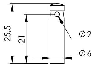
Hohlschraube Threaded bushing
