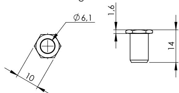
Hohlschraube Threaded bushing
