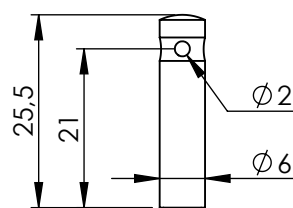
Hohlschraube Threaded bushings
